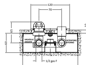
WALL-FIT VALVES WITH THERMOSTATIC HEAD for connections type V14 - H08
