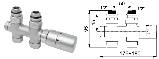
PIPE CENTRES 50 MM STRAIGHT WITH THERMOSTATIC HEAD Only for V7 - V8 - V11 connections type
