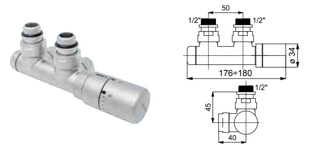
PIPE CENTRES 50 MM SQUARE WITH THERMOSTATIC HEAD (RIGHT) Only for V7 - V8 - V11 connections type
