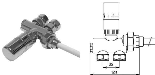
BIDIRECTIONAL VALVE WITH CHROMED THERMOSTATIC HEAD for connections type V12 - V13
