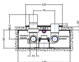
MANUAL WALL-FIT VALVES WITH THERMOSTATIC OPTION for connections type V14 - H08
