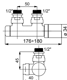
PIPE CENTRES 50 MM SQUARE - WITH THERMOSTATIC HEAD RIGHT - Only for V7 - V8 - V11 connections type
