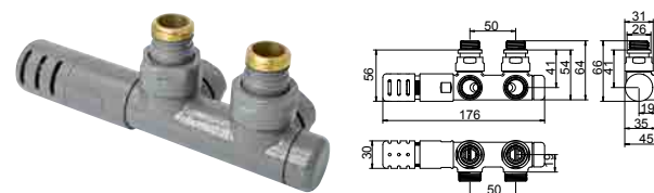
PIPE CENTRES 50 MM SQUARE - WITH THERMOSTATIC HEAD LEFT - Only for V7 - V8 - V11 connections type
