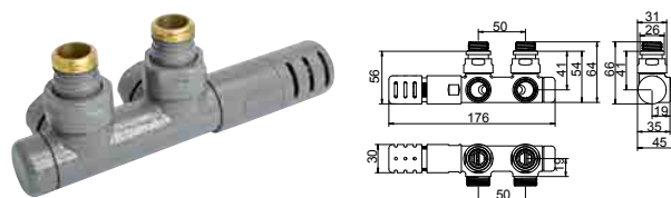
PIPE CENTRES 50 MM SQUARE - WITH THERMOSTATIC HEAD RIGHT - Only for V7 - V8 - V11 connections type
