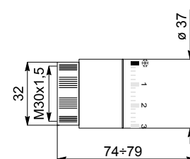
Liquid thermostatic head - WHITE
