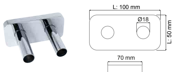
SLEEVING KIT FOR PIPE CENTRES 50 MM
