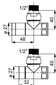
VENTILE ECKFORM MANUELL
