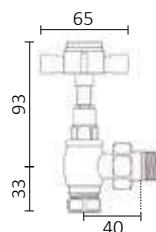
VENTILE ECKFORM MANUELL ANTIKES GOLD
