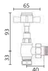
VENTILE ECKFORM MANUELL VERCHROMT
