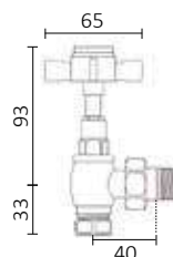
VENTILE ECKFORM MANUELL ANTIKES BRONZE
